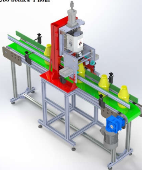
Drilling to chamfer the mouth of the bottle Capacity: 360 bottles/ 1 hour
